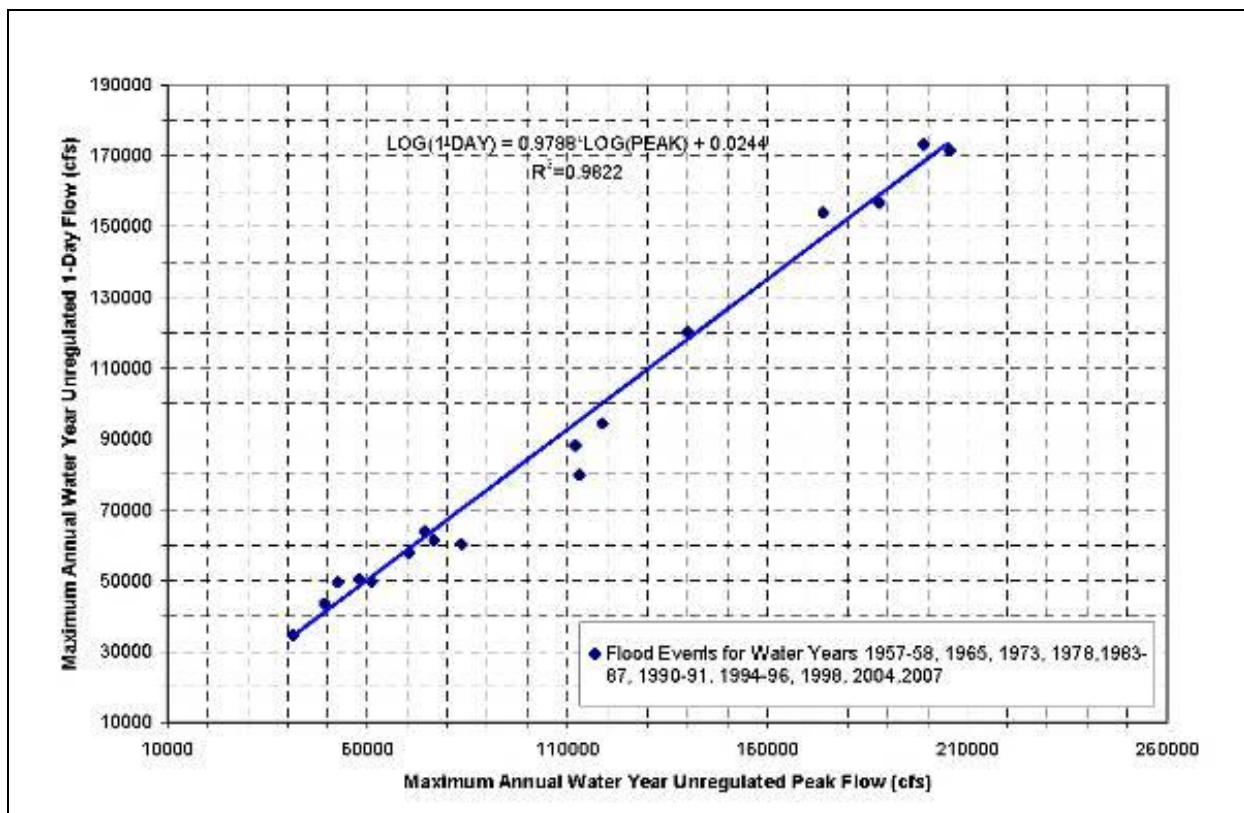
Figure 18. Regression curve of peak to one-day flow for the flood events unregulated by the USACE
