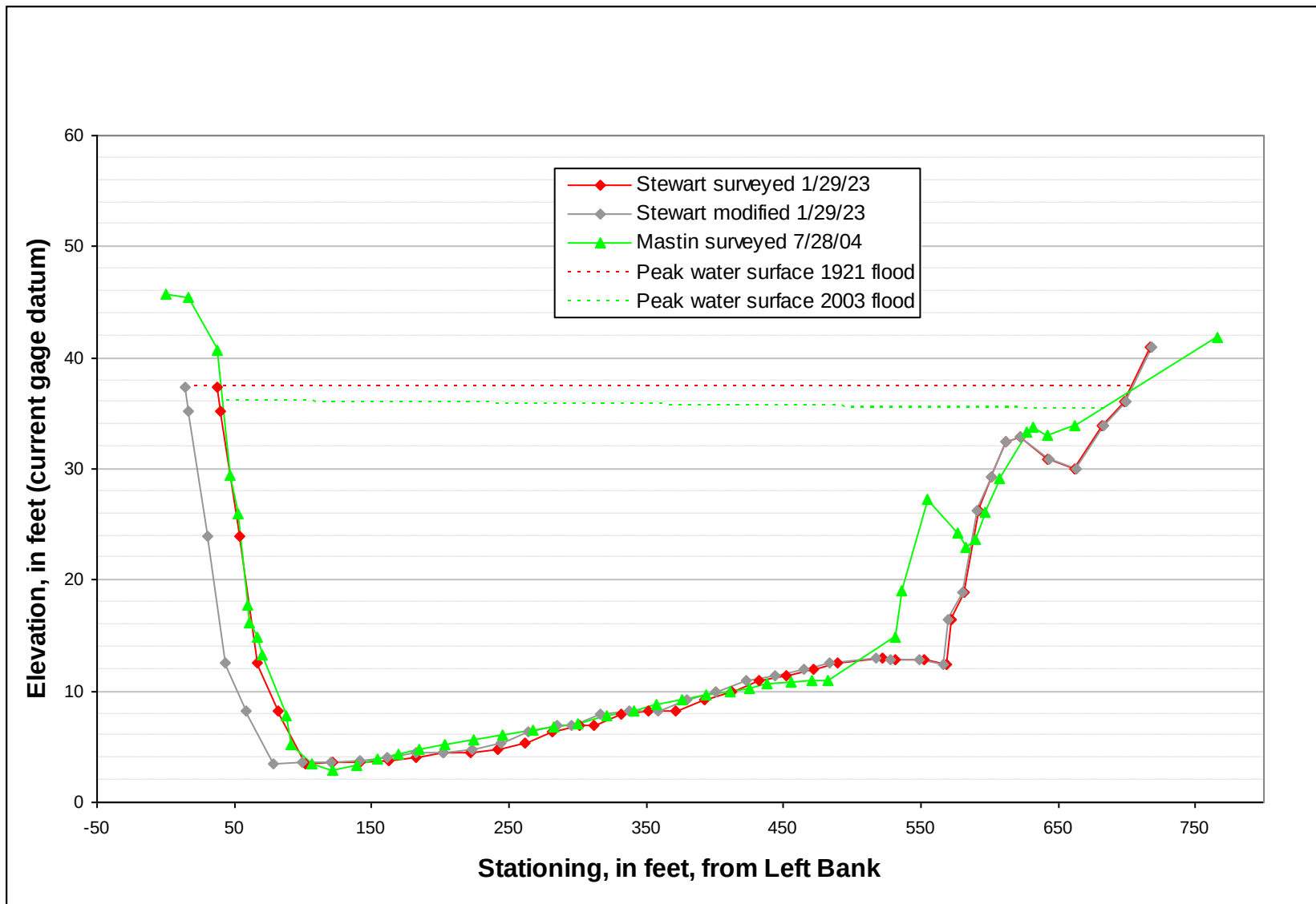
Figure 8. Slope Section XS3 – Skagit River near Concrete, WA
