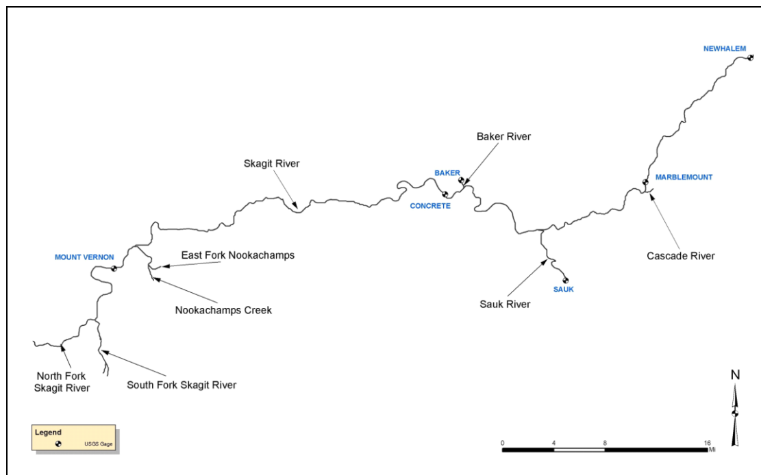
Figure A-1. Skagit River HEC-RAS model routing reaches
