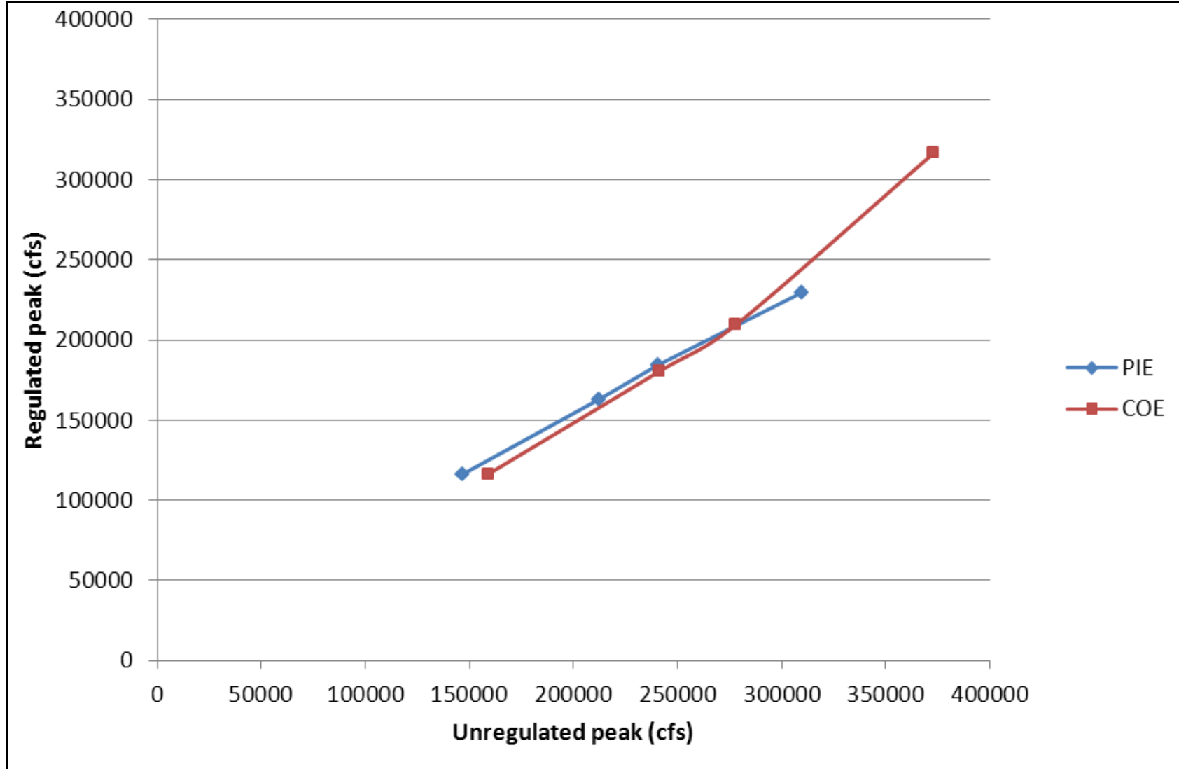
Figure 21. Regulated and unregulated peak discharges at Concrete resulting from the Corps (COE) and PI Engineering (PIE) analyses
